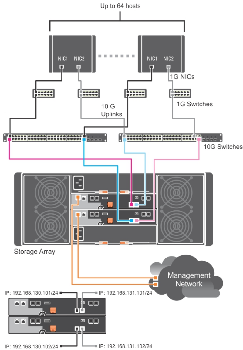
Figure 4. 64 Servers Connected to Two RAID Controllers
