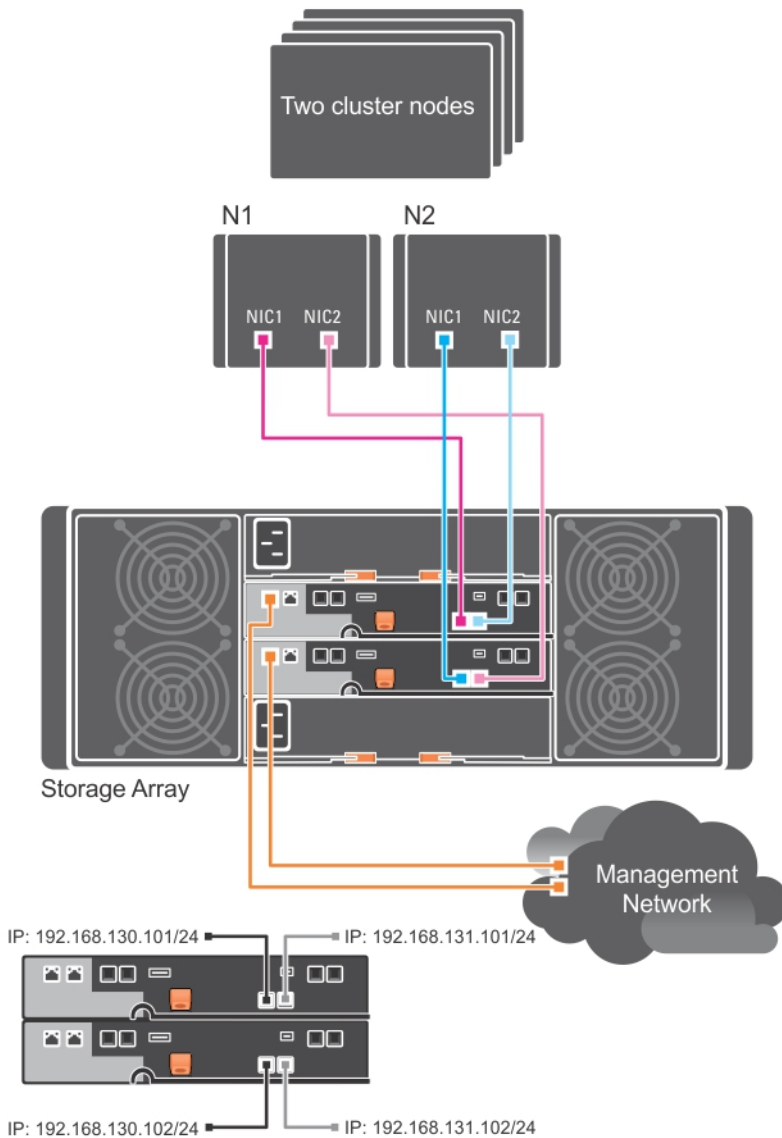
Figure 3. Two Cluster Nodes Connected to Two Controllers
